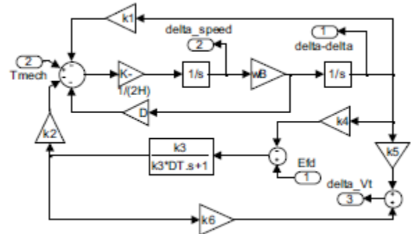
Fig.5.2: overall representation of synchronous machine
