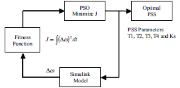
Fig.4.2: Design procedure with PSO
