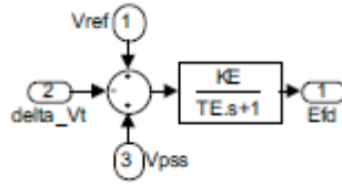
Fig.5.3: Simulink layout of excitation system
