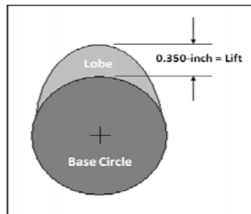
Fig1.4: lobe height
